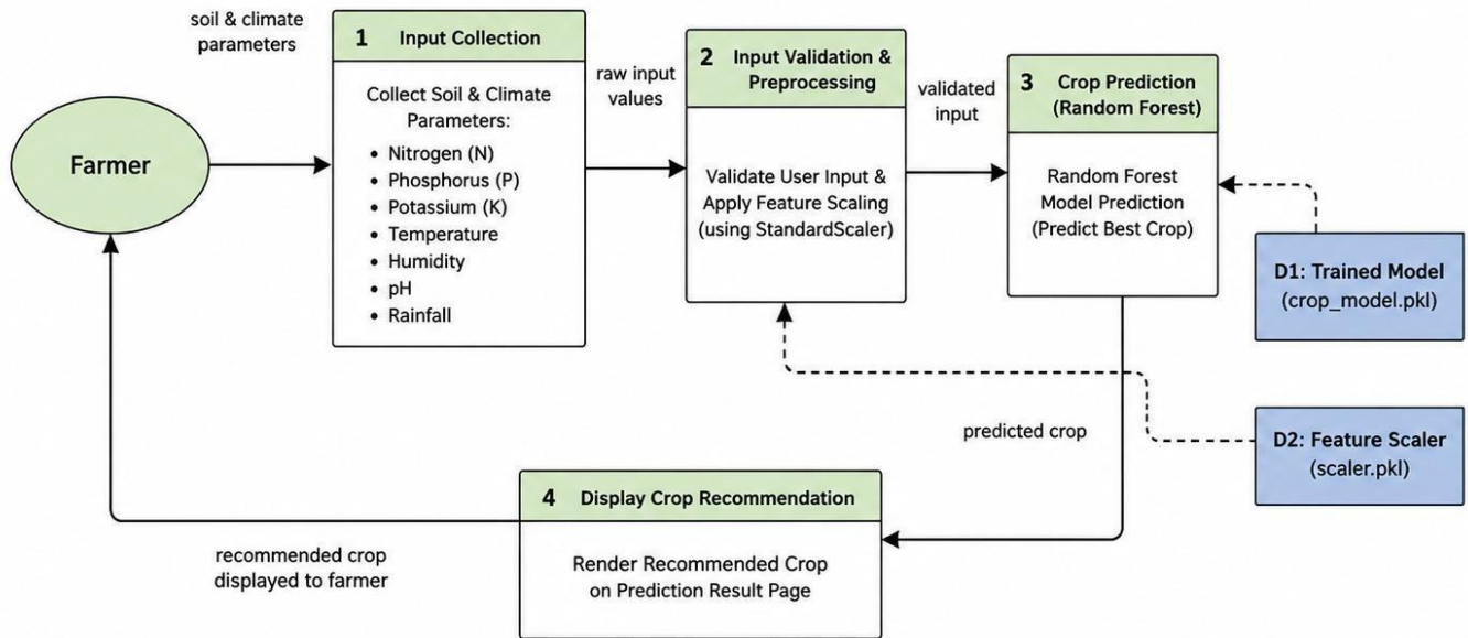
Figure 1: Level 0 DFD for OptiCrop: Smart Agriculture Production Optimization Engine
